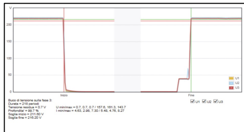
MONITORAGGIO POWER QUALITY
